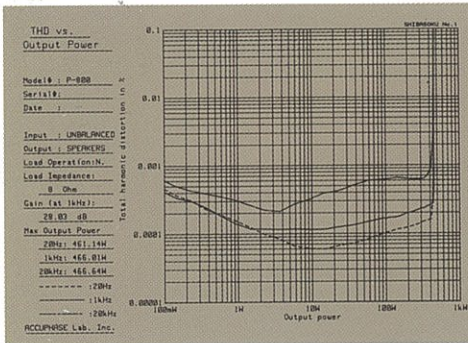
● OUTPUT POWER vs. TOTAL HARMONIC DISTORTION (at 8 ohms, NORMAL IMP mode)
